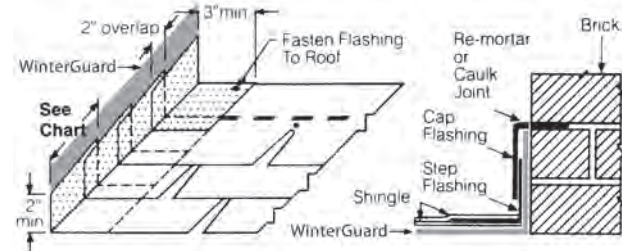
Figure 6-2: Sidewall step flashing (see also Figure 6-10).
