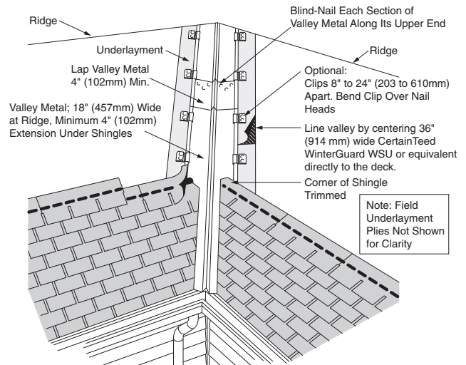
Figure 6-20: Typical open valley attached by cleats.
