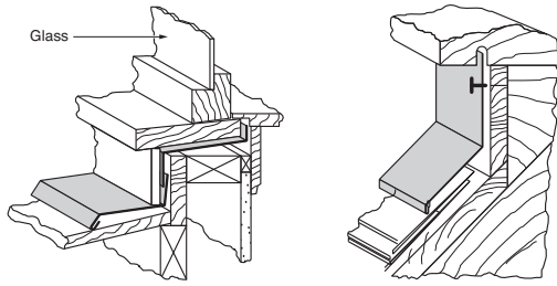
Figure 6-15: Two examples of base flashing below the window sill of a dormer.
