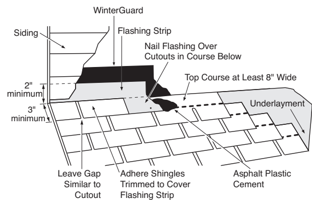
Figure 6-3: Front wall flashing.
