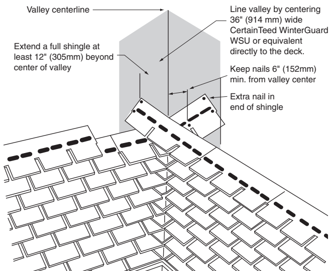
Figure 6-19: Woven Valley Application.
