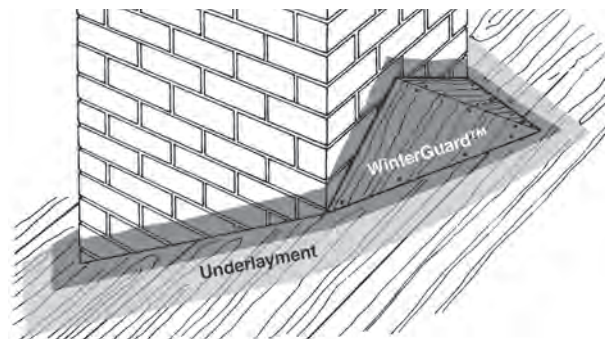
Figure 6-8: Chimney through the roof deck.
