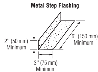
Figure 15-23: Metal step flashing.
