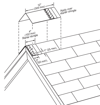
Figure 15-20: Apply a full cap shingle over the starter shingle.
